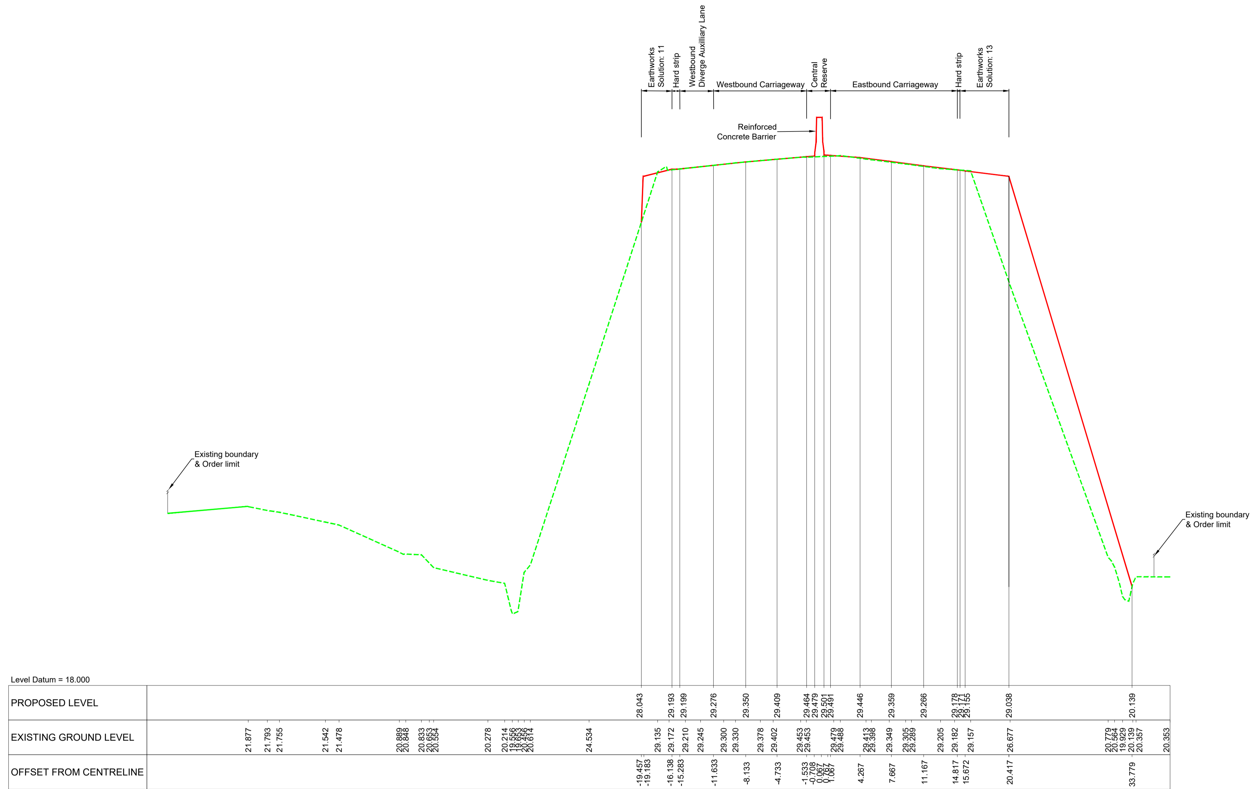
Junction 6 Westbound Off-Slip & Eastbound On-Slip Chainage 25500.0000 Work No. 16c & No. 16b Works Plan Sheet 22
